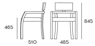
Sedia 1840 chair, Stuhl
