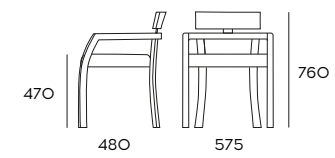
Sedia 1860 chair, Stuhl
