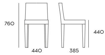
Sedia Essential 1910 chair, stuhl
